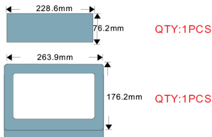
13 PICTURE FRAME & RISER
