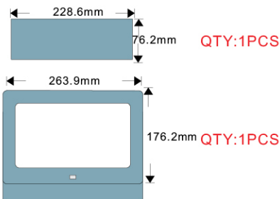
12 VIDEO FRAME & RISER
